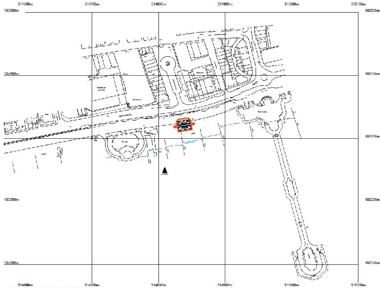
© Crown Copyright and database rights 2018 OS 100019990 LOCATION PLAN FOR PROPOSED OBSERVATION WHEEL @ 1:1250
